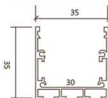
605-35M Coller
