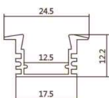
505-11M DEEP COLLER
