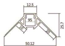
705 Outside Corner
