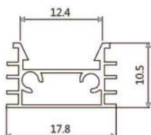
418-10.5MM DEEP COLLERLESS FURNITURE
