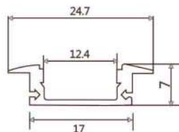
408-6MM COLLER
