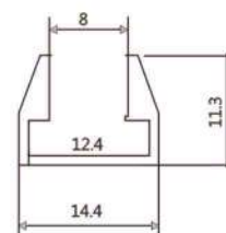
539- Glass Shelf
