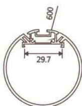
600 MM Round Suspended
