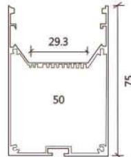
607 50x75 Hanging
