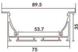
608A 75x35 Deep Coller
