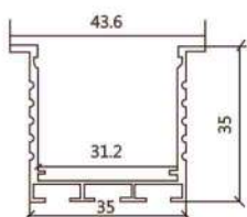
603(A)-35MM Coller
