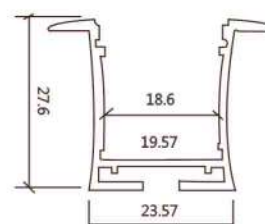
602(A) 25x25MM Coller
