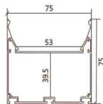
608-1 75x75 Hanging
