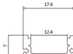
409-6MM COLLERLESS
