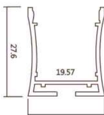
602 25MMx25MM Collarless
