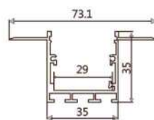
706 35mm Trimless
