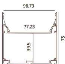
609-1 100x75 Hanging
