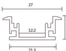
532A Footmounted
