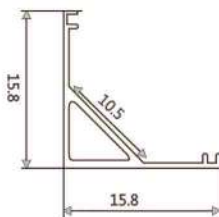
501 CORNER 16×16
