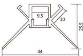
704 Trimless Inside Corner
